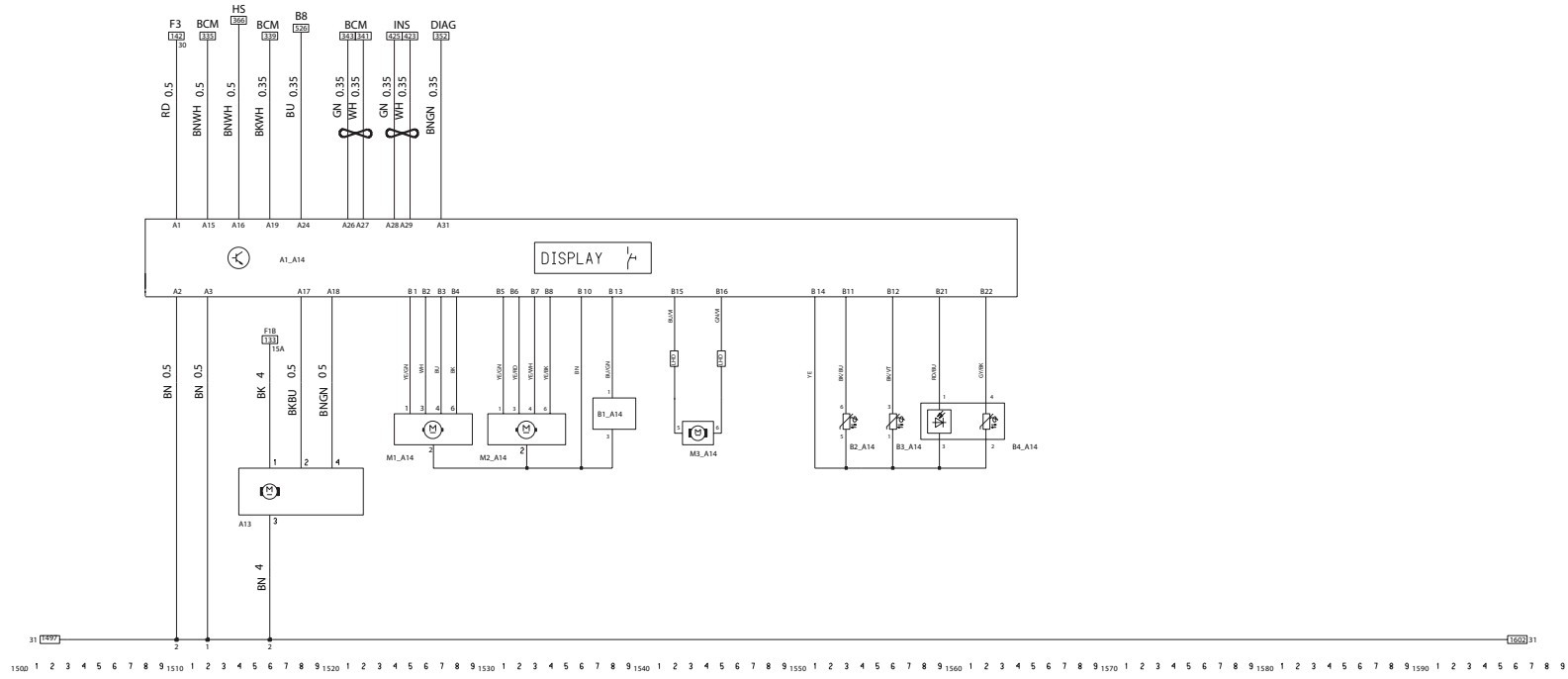
BLOWER PASSENGER COMPARTMENT, ELECTRONIC CLIMATE CONTROL (ECC)
